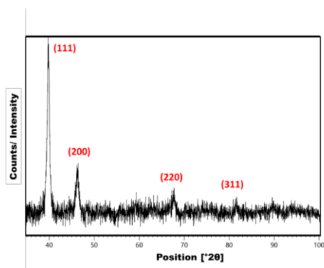
Fig. 4. XRD pattern of PdNPs
